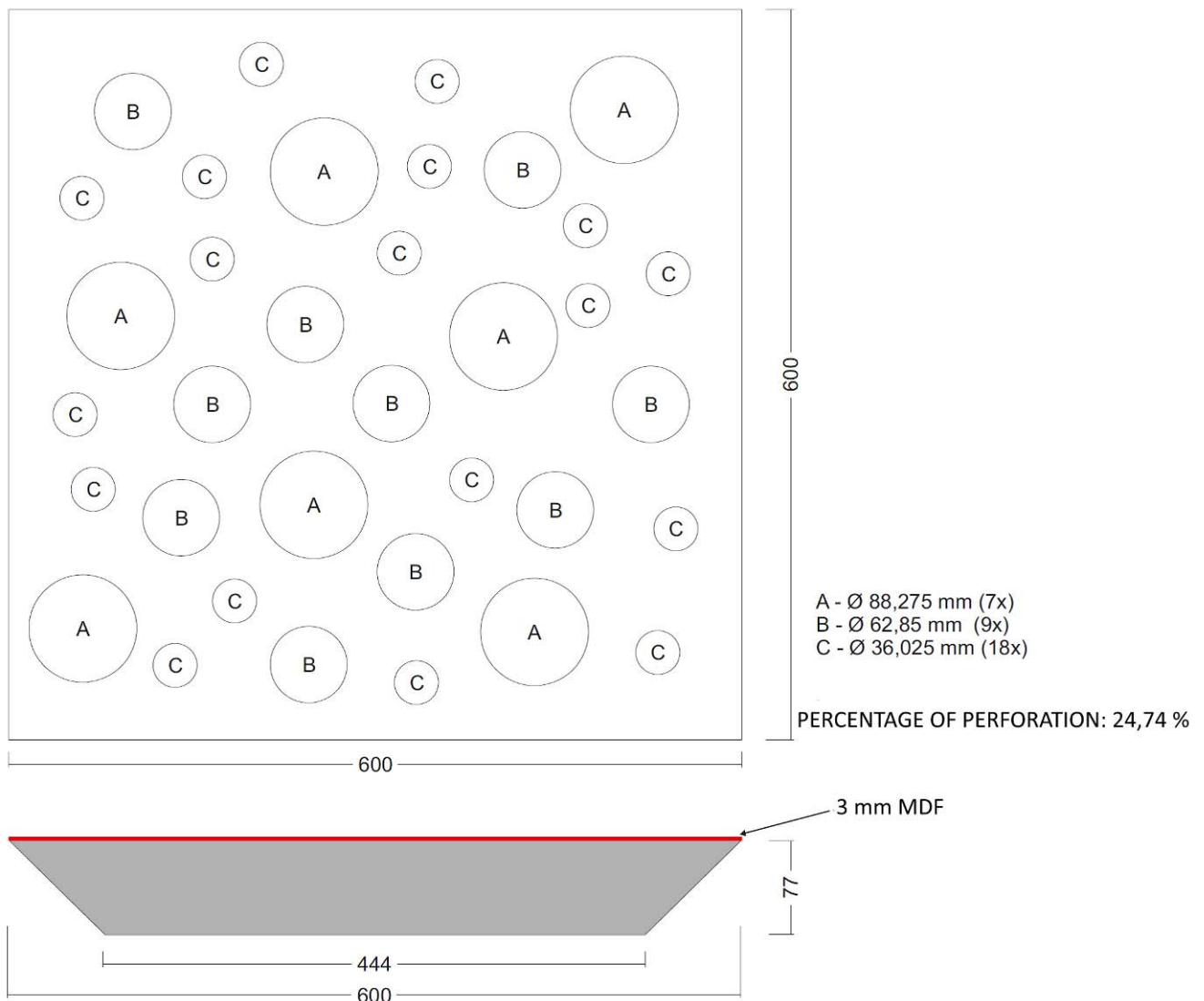
Picture 1: schematic drawing of the Decosorber Dot 8 sound-absorption cladding.
